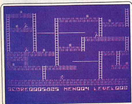
Lode Runner
